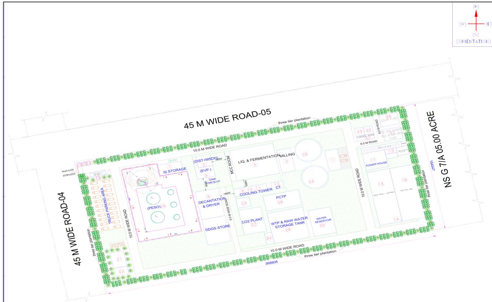
Figure1: Site Layout
