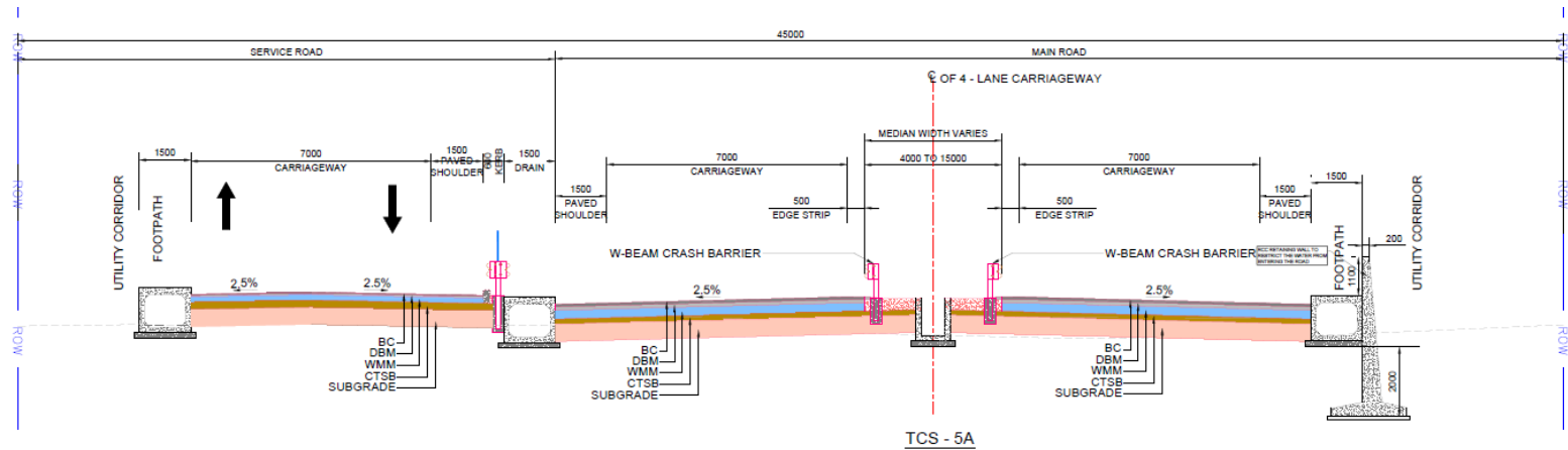
TCS - 5A TYPICAL CROSS SECTION FOR 4-LANE CARRIAGEWAY AT APPROACH LOCATION WITH LHS SERVICE ROAD APPLICABLE IN RUB SECTION
