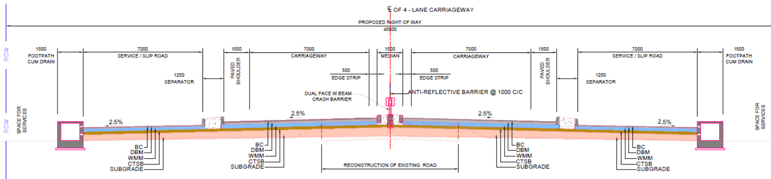
TCS - 6 TYPICAL CROSS SECTION FOR 4 LANE CARRIAGEWAY WITH SERVICE ROAD AT RECONSTRUCTION LOCATION (RECONSTRUCTION OF EXISTING ROAD)
