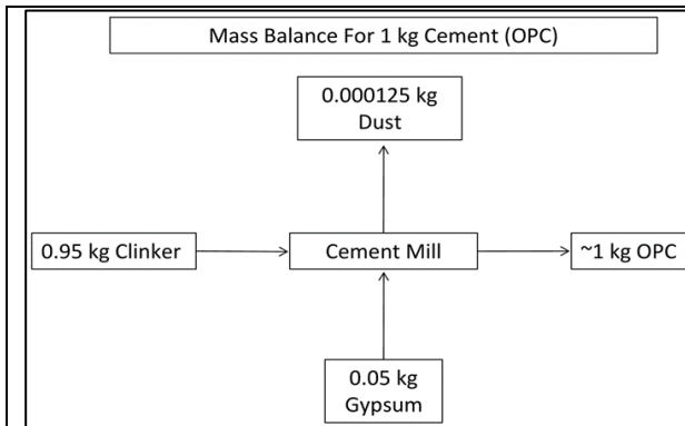
Figure 2.0(a) Mass balance diagram of OPC
