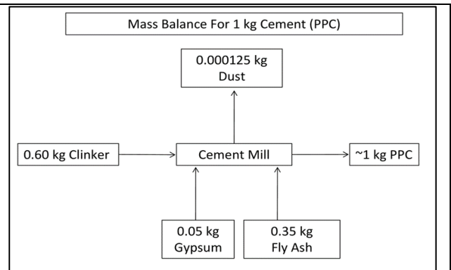
Figure 2.0(b) Mass balance diagram of PPC
