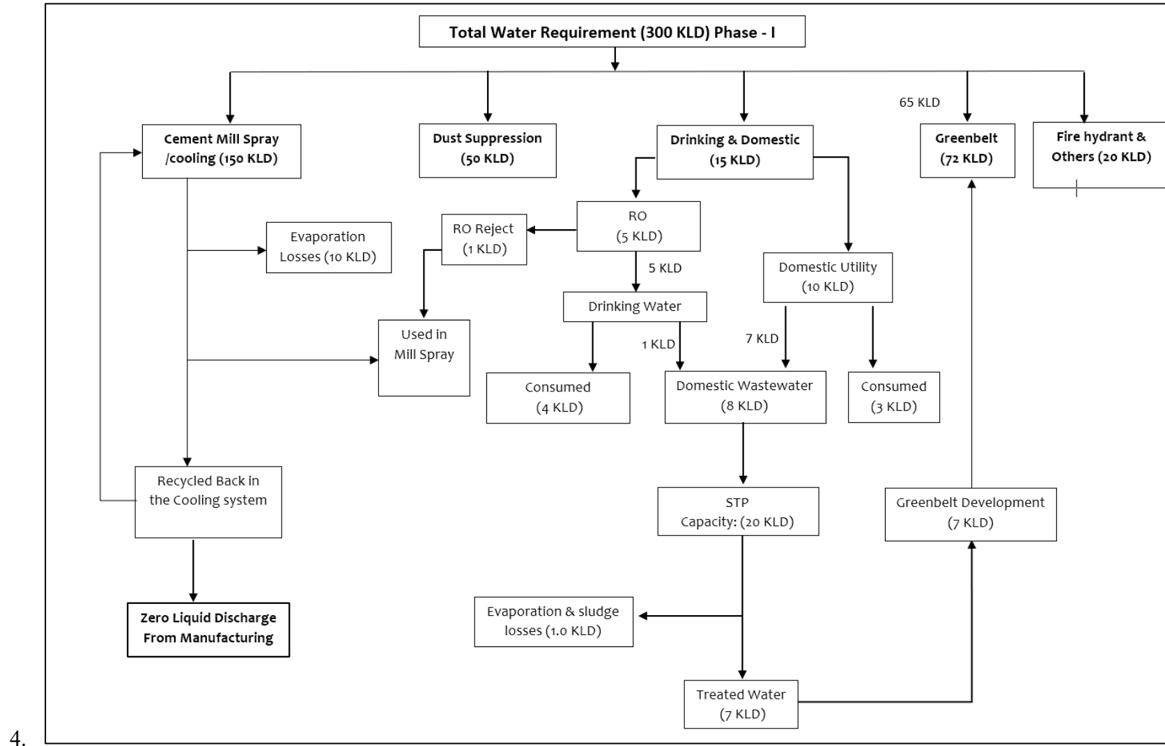
Figure 3: Water Balance for total water requirement for Phase - I
