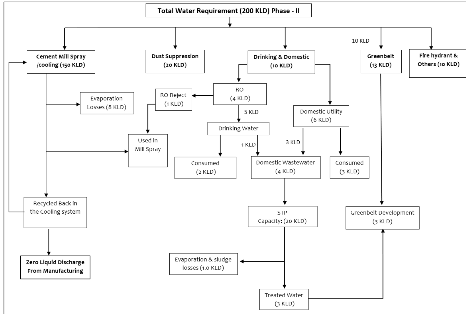
Figure - 4 Water Balance for total water requirement for Phase - II
