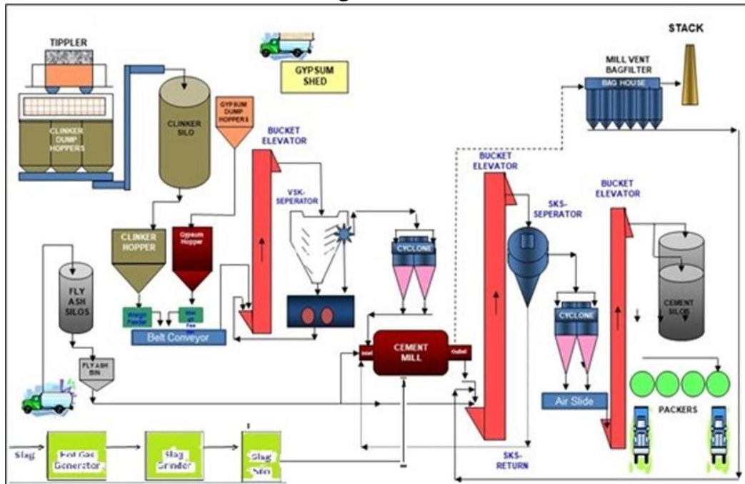
Figure 1.0: Schematic Process flow Chart of Grinding Unit
