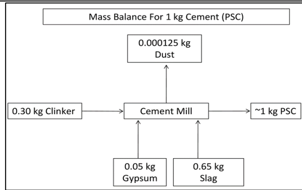
Figure 2.o(C) Mass balance diagram of PSC
