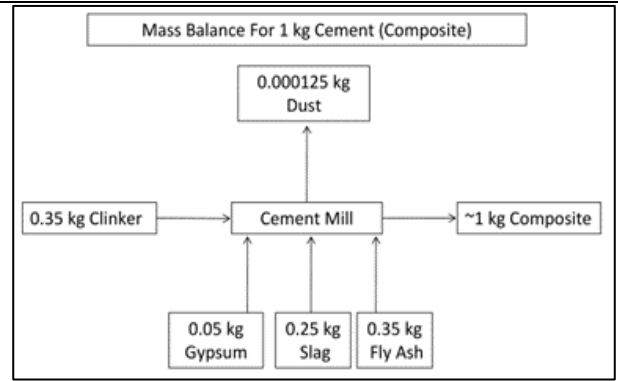
Figure 2.o(d) Mass balance diagram of Composite Cement
