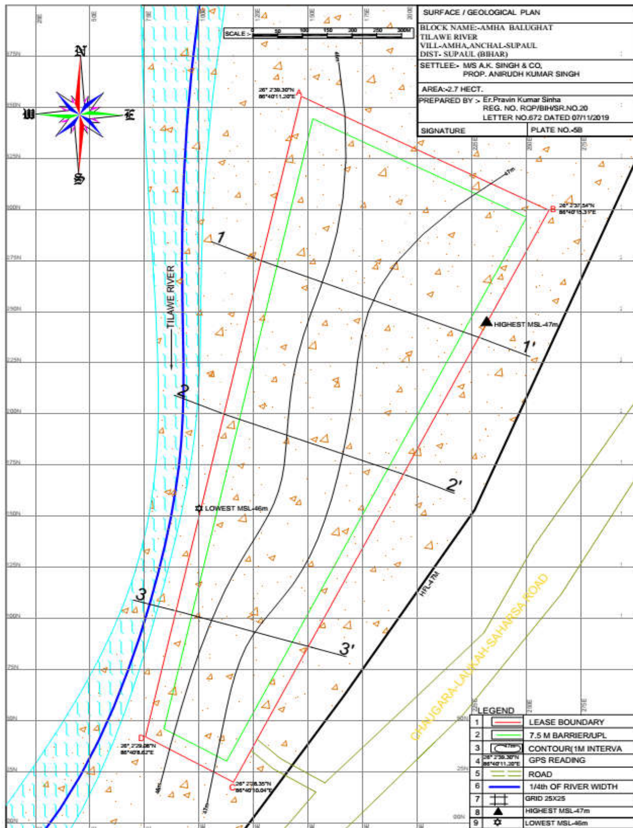
SURFACE/ GEOLOGICAL PLAN
