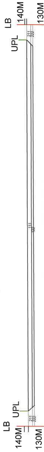
SECTION ALONG 3-3'
